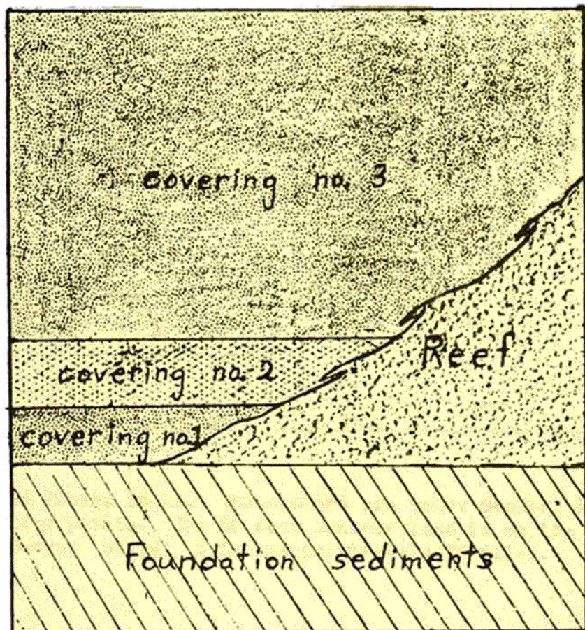
Fig. 1. Diagram of a buried Canadian atoll reef, with evaporite coverings. No. 1--laminated anhydrite (80 feet), no. 2--laminated dolostone (70 feet), no. 3--anhydrite and dolostone in alternating layers (500 feet thickness). These coverings belong to the Middle Devonian Period.
